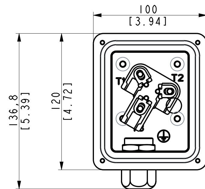
TERMINAL BOX LAYOUT SCALE 1:2
