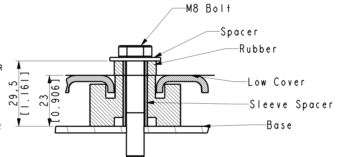
DETAIL FOOT
