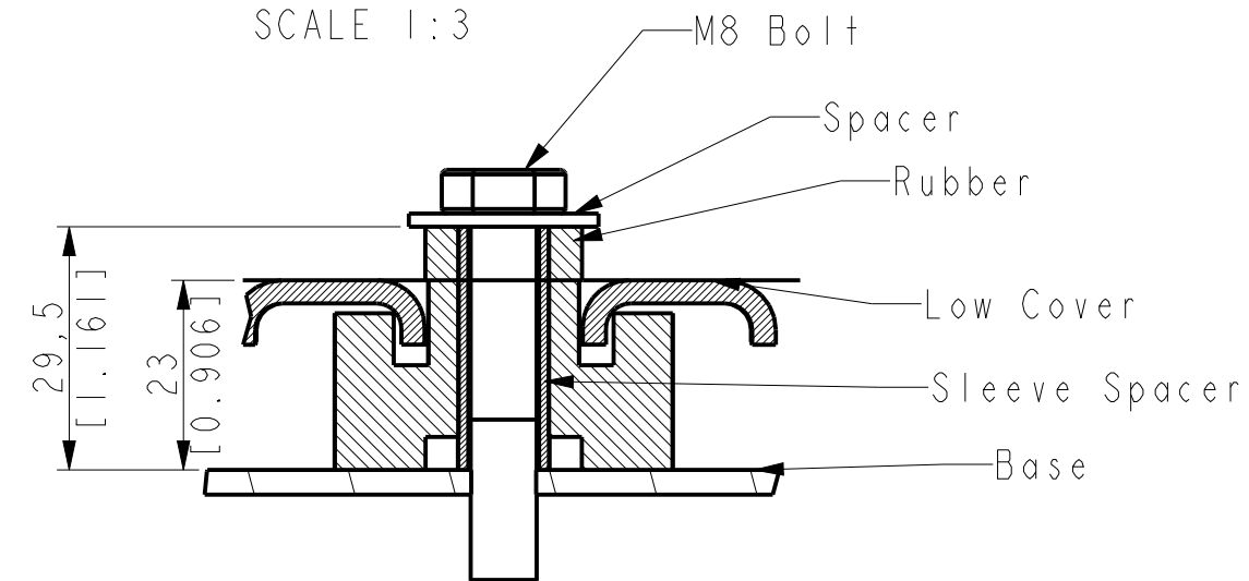
DETAIL FOOT
