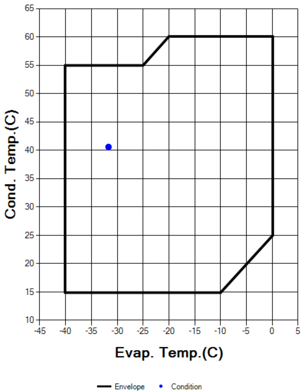
Envelope XFL72B-D1-105
