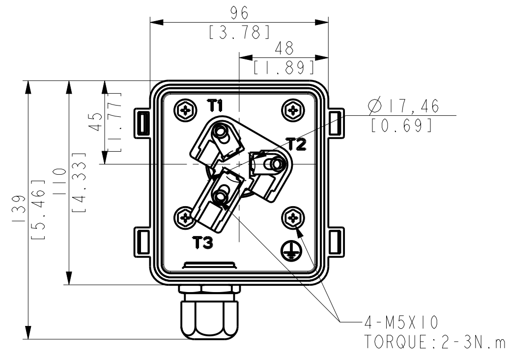
TERMINAL BOX LAYOUT SCALE 1:3
