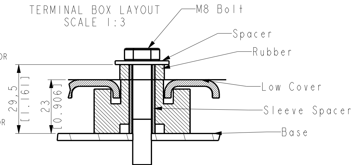
DETAIL FOOT
