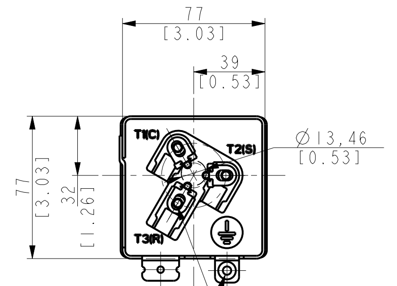
TERMINAL BOX LAYOUT SCALE 1:2 TORQUE: 2-3N.m
